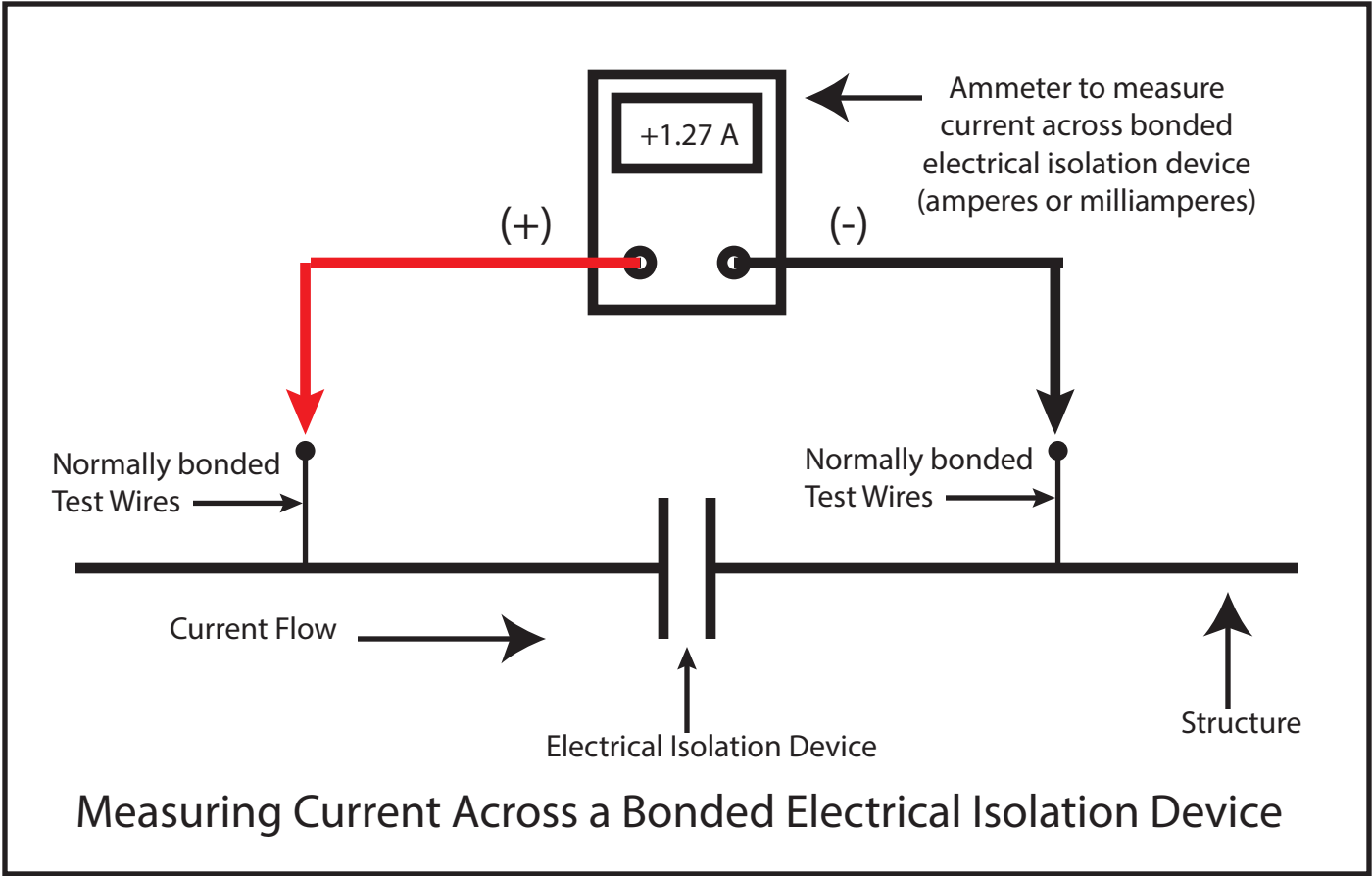
Measuring Current with an Ammeter Figure 6-13
