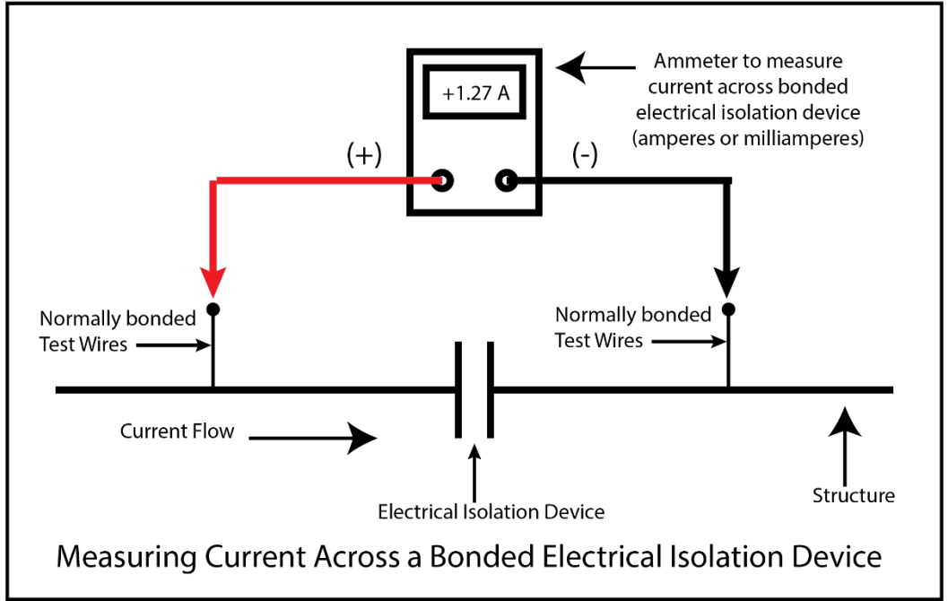
Measuring Current with an Ammeter Figure 6-13
